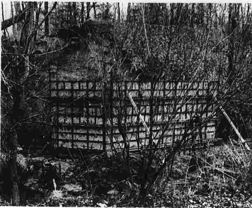
Storm Drainage Project A concrete wall has been installed to help with the installation of storm drainage piping in the St. John Street area of Manchester. The wall has been installed to retain the earth berm behind it and to prevent the stream from overflowing and eroding underneath the pipe installation.
